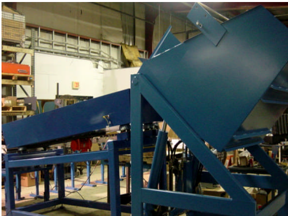
Heavy Duty Receiver Pan Feeder w/ active pan for receiving parts dumped from portable bulk containers. Pan absorbs impact load and is integrated to dumper to effectively meter parts to "on demand" upstream systems.
