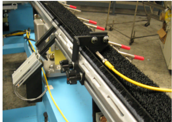
Walking Beam Escapement
