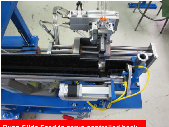
Dyna-Slide Feed to servo controlled back stop and pick and place loading precision Nest position.
