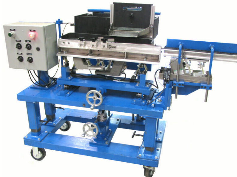
Model Shown: Centerless Grinder Feeder-Portable Model 1436 w/Space Saver Supply Hopper & Standard Base with X & Z Adjustment
