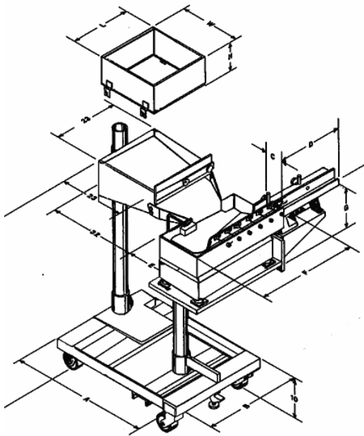
Pedestal Mounted Feeder w/ Supply Hopper
